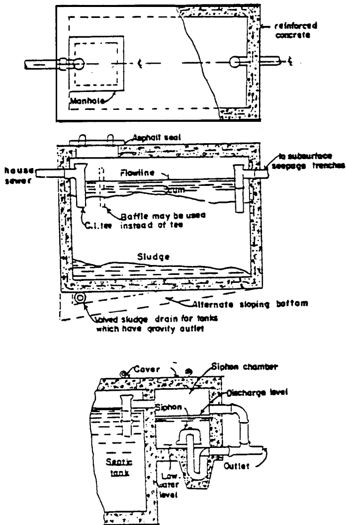
Figure 7-2. Typical septic tank
